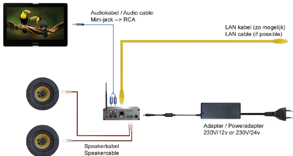
Wiring diagram Wi-Fi audio sets
