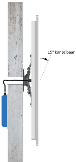
Side view: TV mounted with VESA wall mount.
